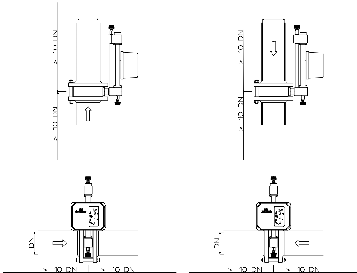
Type TMW line mounting examples
